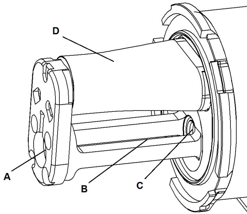
Figure 1-4: GS01 measuring cell details
